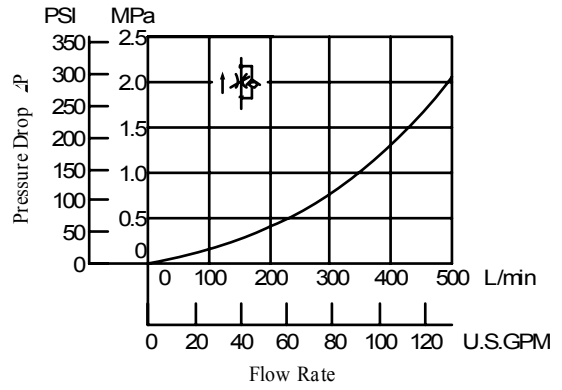
Pressure Drop at Throttle Fully Open
