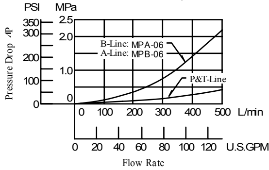
Pressure Drop
