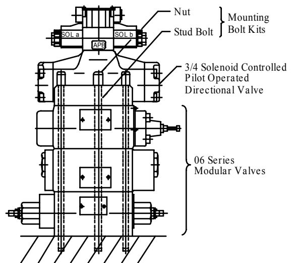
06 Series Modular Valve Assembly
