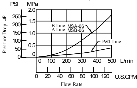
Pressure Drop
