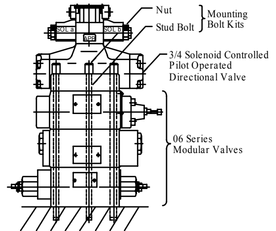
06 Series Modular Valve Assembly
